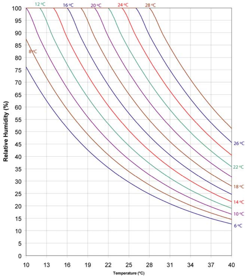
Constant Dew Point Lines for Ambient Temperature and Relative Humidity
